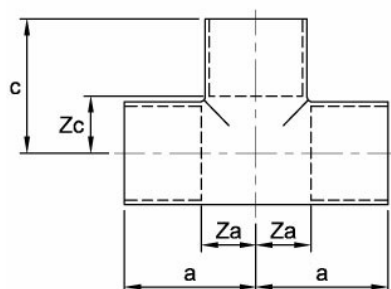
N24 Tee
